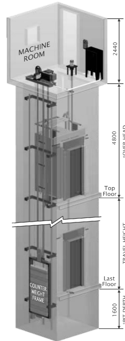
LIFT WELL
