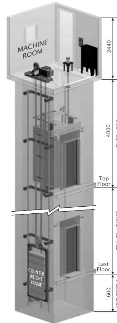
LIFT WELL
