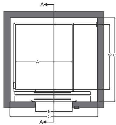
LIFT SHAFT, CAR, & C.W. PLAN
