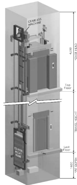
LIFT WELL
