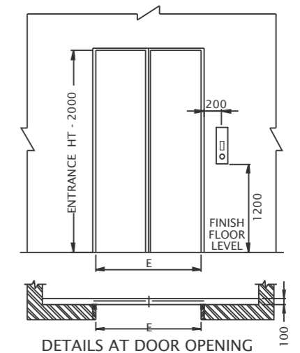
DETAILS AT DOOR OPENING
